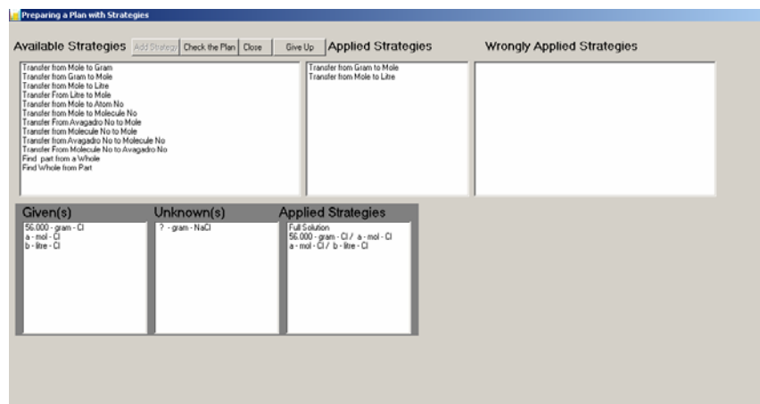
Figure 4: Preparing a Plan in the Polya Problem Solving Mode of Mole Solver
