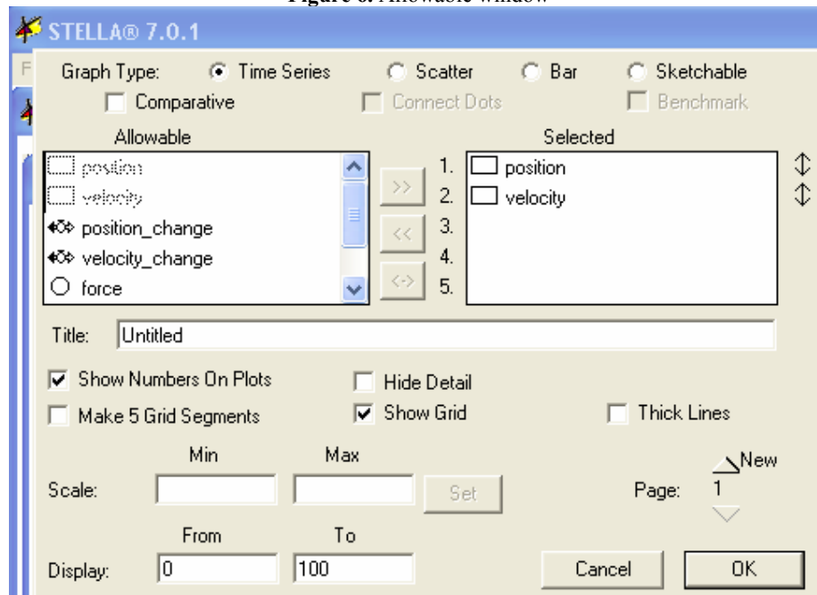
Figure 7. Selected window
